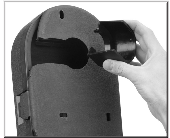
Figure 18. Installing the bearing guard.
